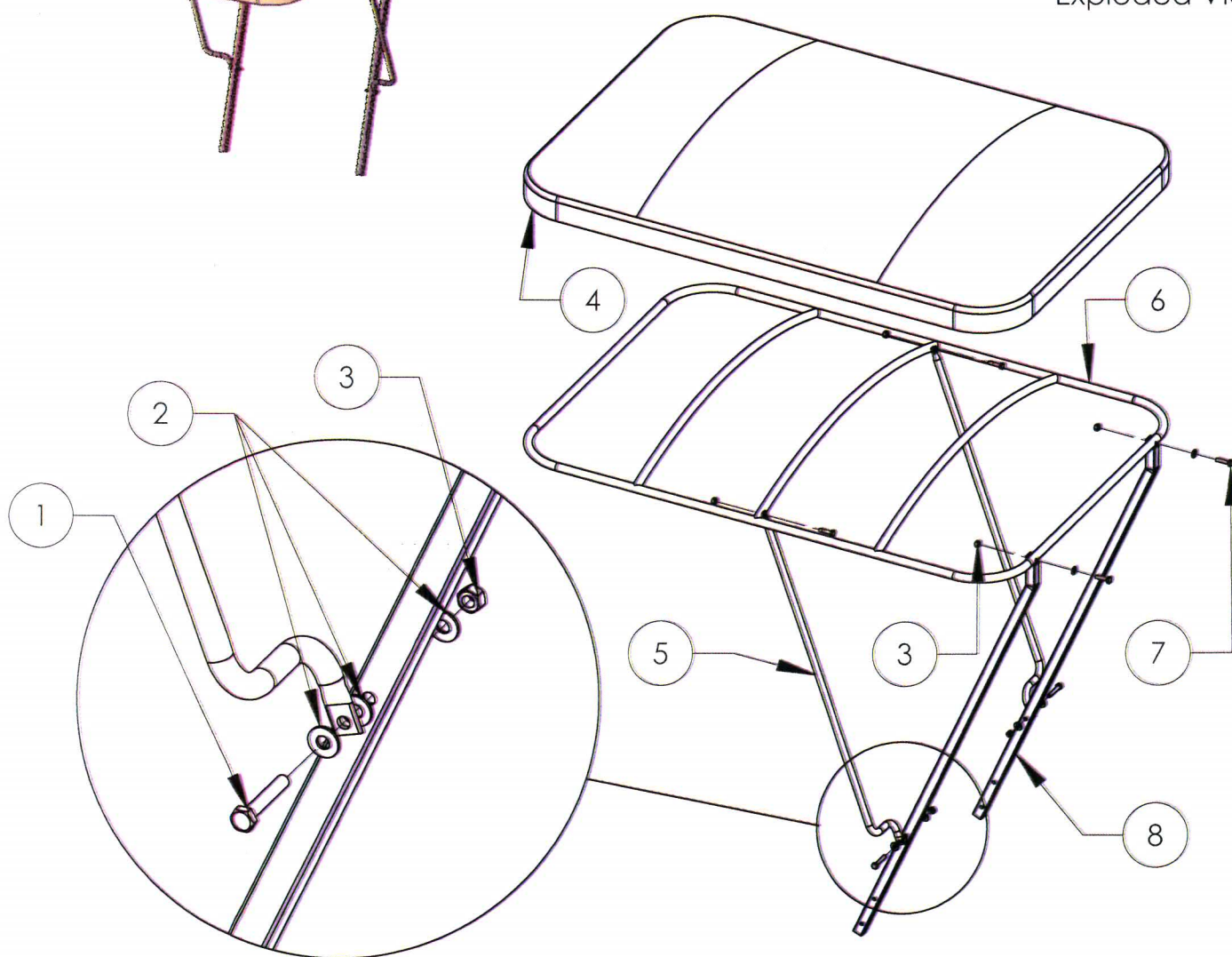
Exploded View
